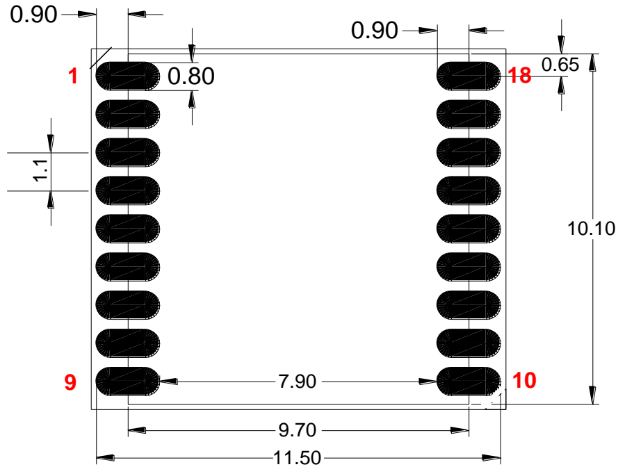
Figure 25: Recommended Footprint
